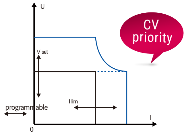
High-speed and seamless battery charging and discharging without overshoot (CV-High,CC-High,CCpriority)
